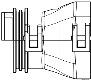
CLOSED (MOUNTED) CONDITION 2357302-1 AS SHOWN
